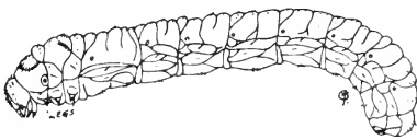
Fig. 346. Eupsalis minuta Drury.
